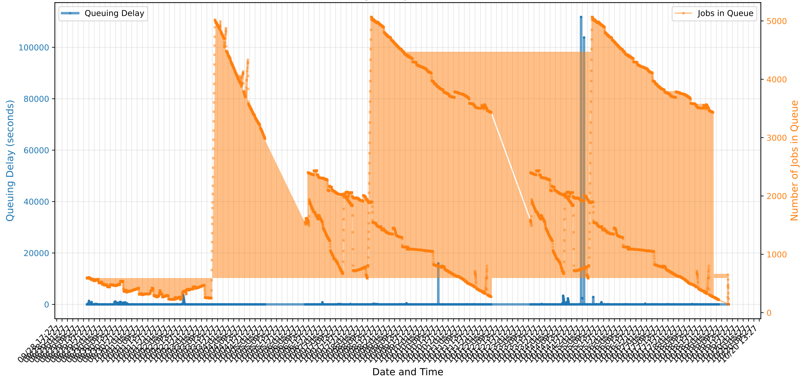
UGE Cluster Queuing Delay Over Time for 4 Core Jobs
